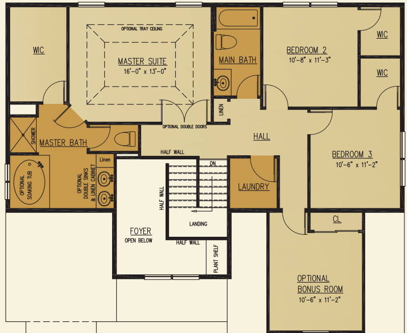
2nd floor
